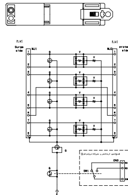
Basic Circuit Diagram
